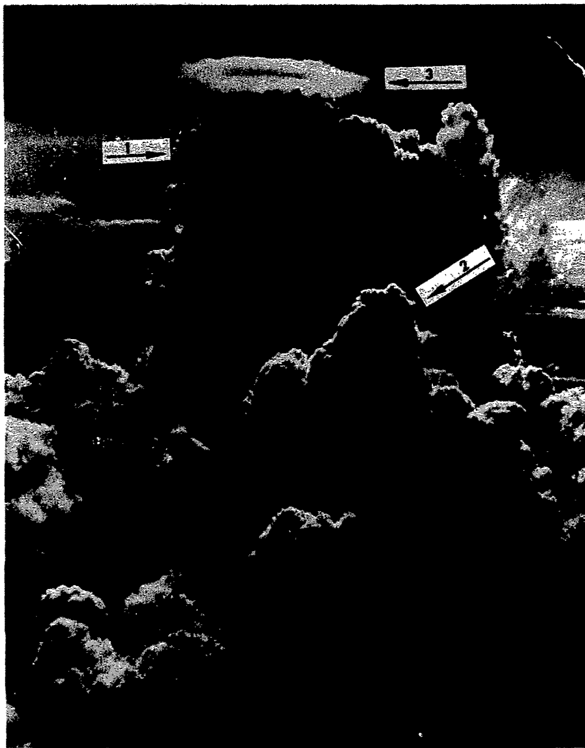
Figure 20. Spectacular Cloud Development Followed Seeding Operations on 12 June. At the time of seeding, about 20 minutes prior to the time of this photograph, the target cloud complex (1) was only the same size as the towering cumulus (2) in the foreground. The pileus cap (3) is a good indicator of vigorous cloud development.
