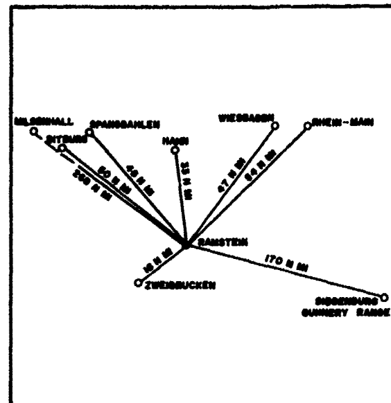
Figure 8. European Locations at Which Airborne Seeding with Dry Ice Took Place in 1970-71. All seeding aircraft operated from Ramstein AB, Germany.
